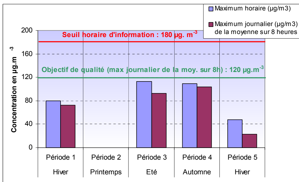
Figure 4.6.5.7 : Concentration d'ozone (O 3 )
